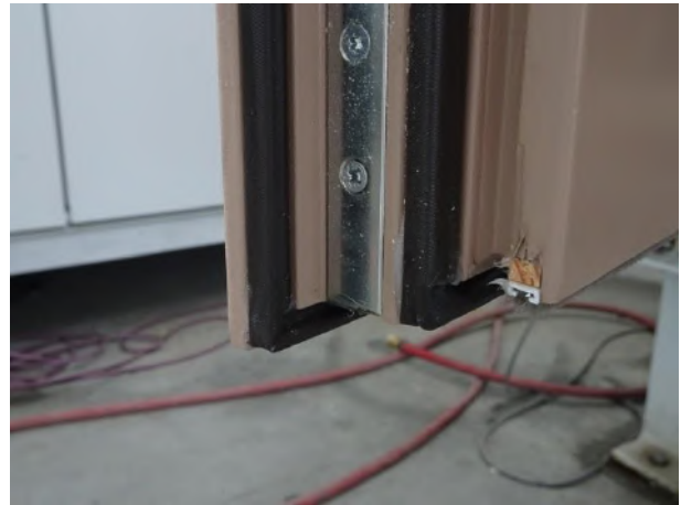
Picture 14 Leaf seal at bottom
